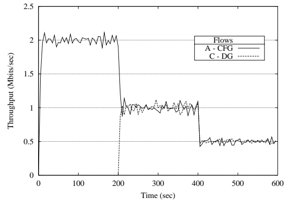
Fig. 9. Scenario 2, Simulation: Throughput with delayed senders
