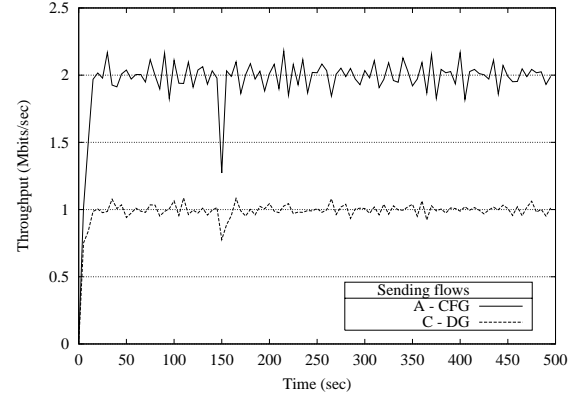
Fig. 4. Scenario 1, Simulation: Throughput
