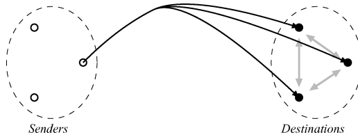
Fig. 13. Destinations agreement algorithms.
